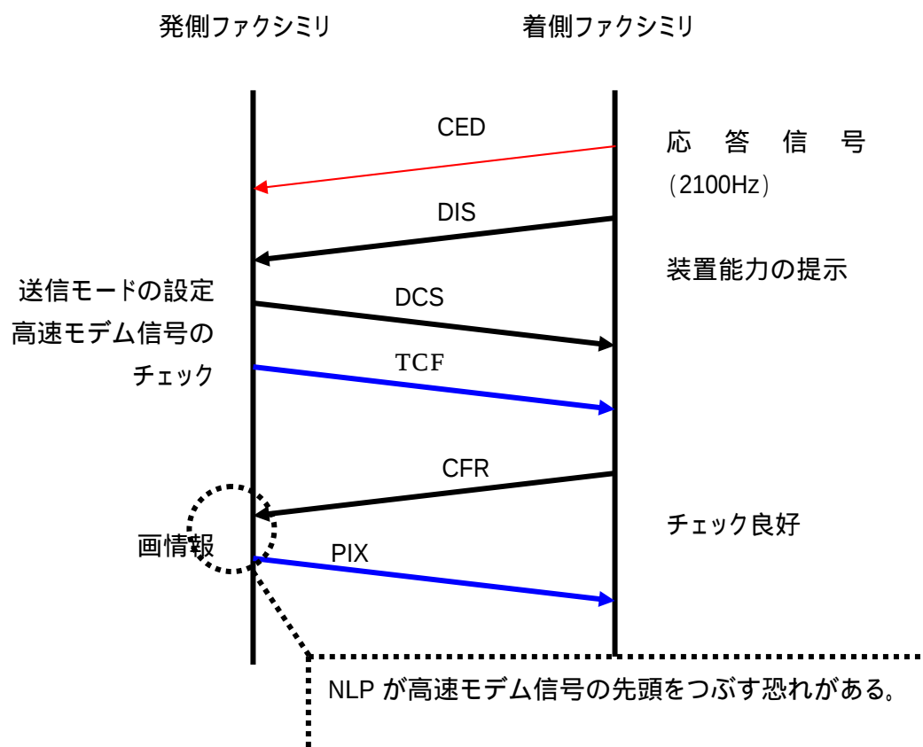
図表3.5 NLP(Non-linear processor)動作フロー
